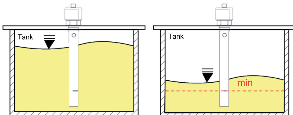
Fig. 3: Installation options
