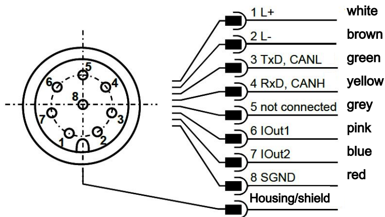
Fig. 5: Sensor plug pin assignment
