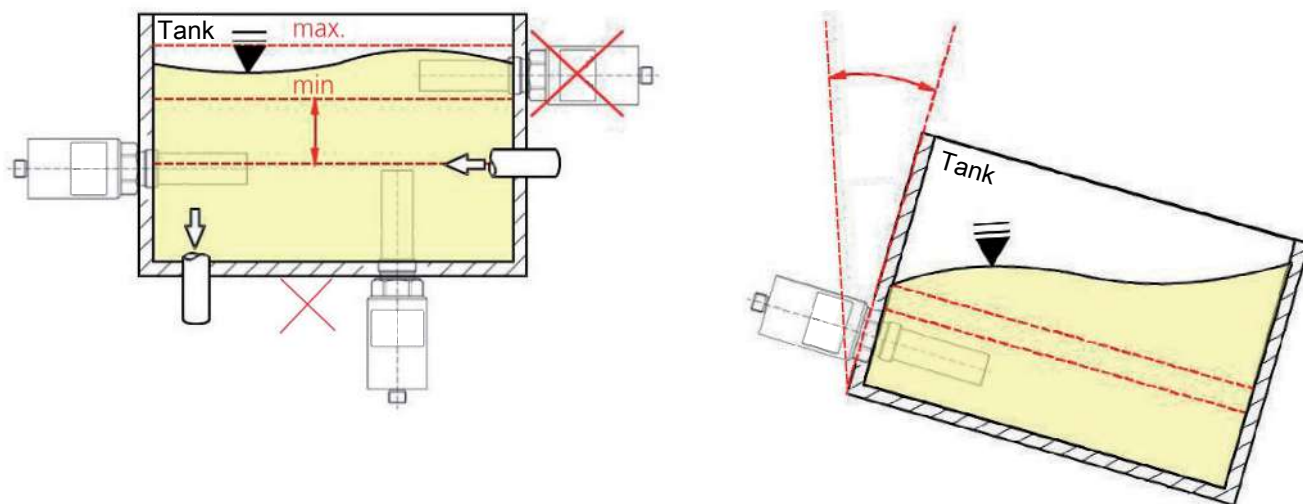
Fig. 4: Installation recommendations
