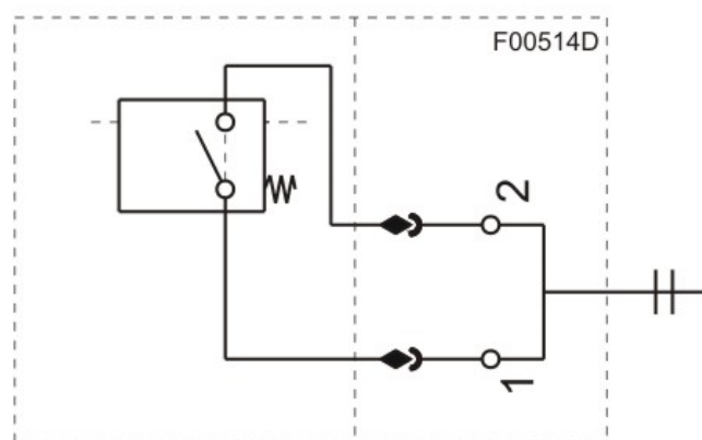
Fig. 2: Pin assignment for type Mahle PIS 3085/2.2
