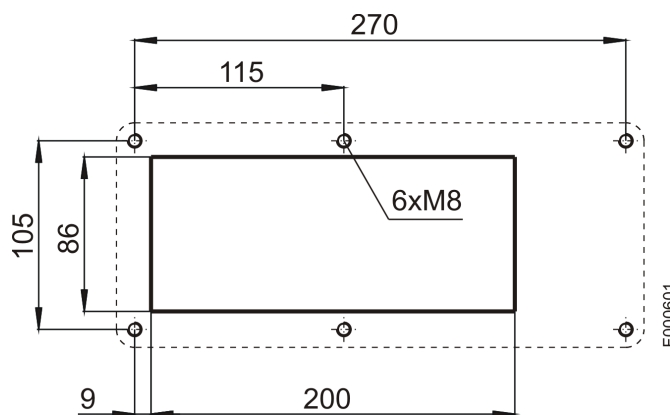
Fig. 1: Hole pattern for MT installation opening
