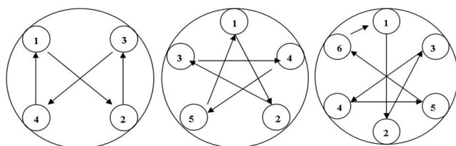
Four screws
