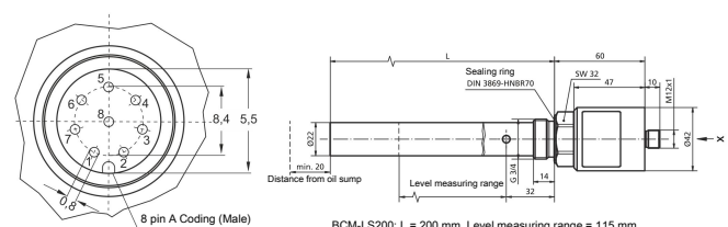
Connection dimensions BCM-LS200
