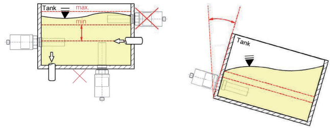
Fig. 3: Installation recommendations
