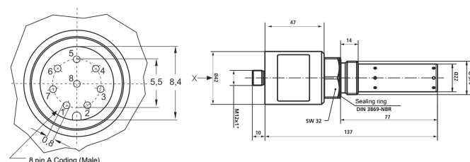
Connection dimensions BCM-MS200
