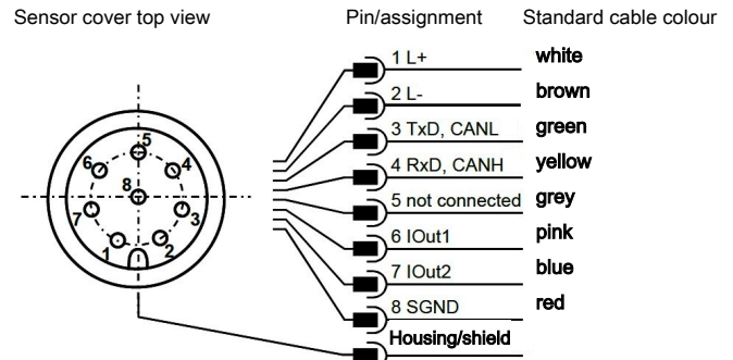
Fig. 4: Sensor plug pin assignment
