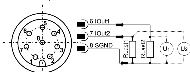
Fig. 6: Connecting the load resistances to measure the analog 4..20 mA outputs
