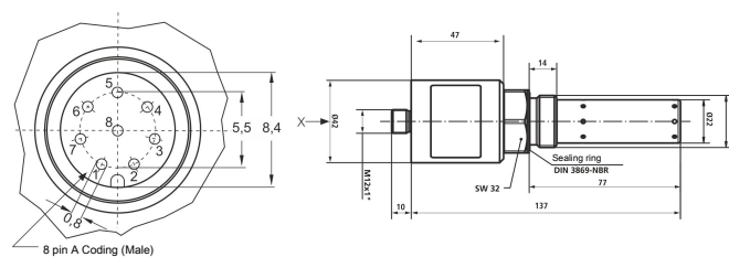
Connection dimensions BCM-MS200
