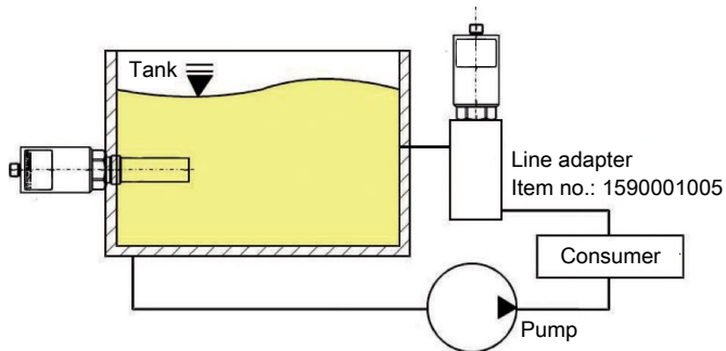
Fig. 1: Installation options
