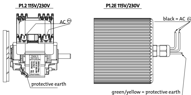
Fig. 2: Electrical connections P1.2 pumps
