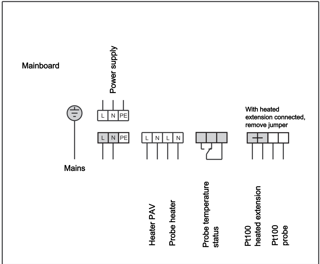
Fig. 1: Connection Diagram
