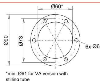
Flange drawing
