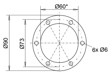
Flange drawing
