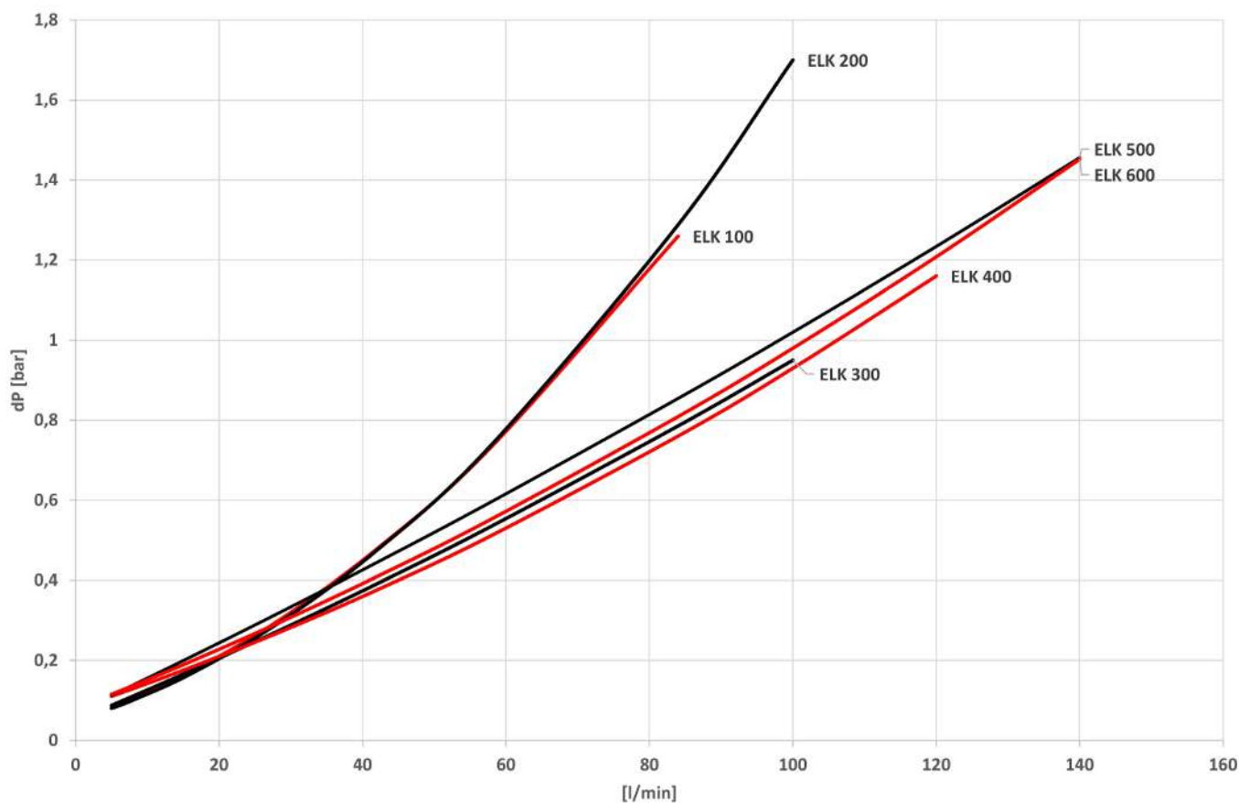
Fig. 2: Pressure loss
