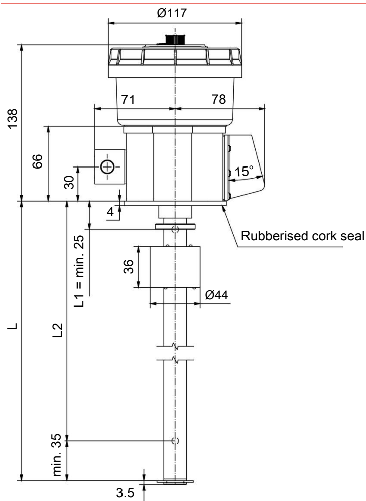
Basic version
