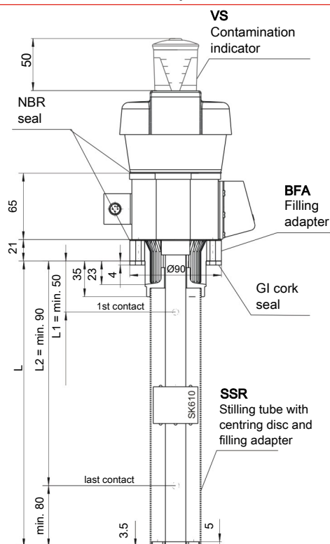
With options
