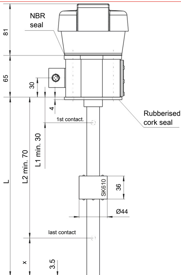
Basic version
