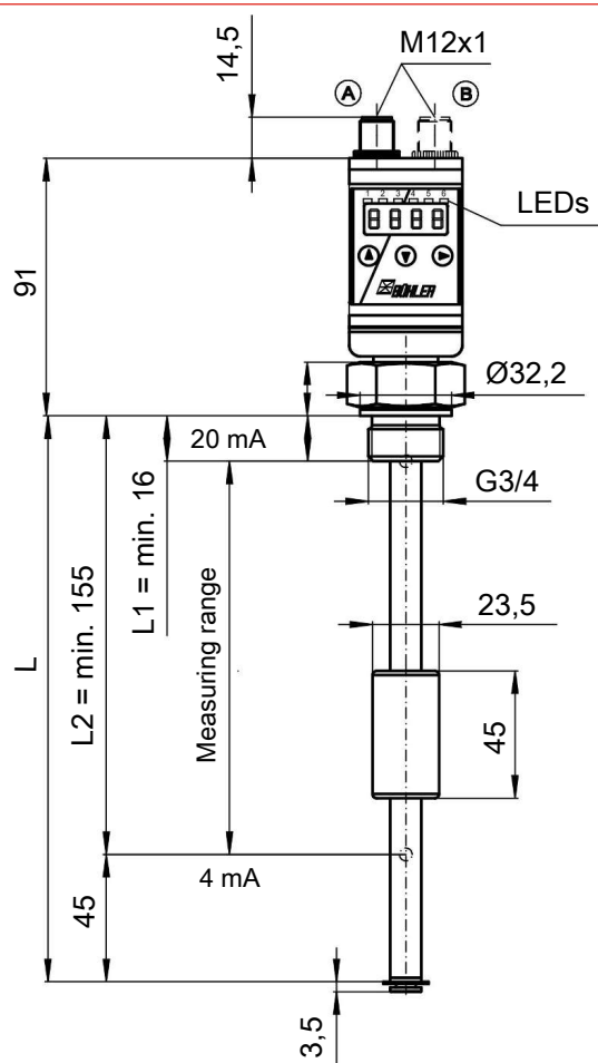
Basic version
