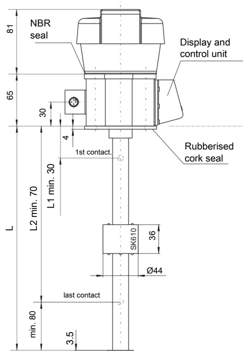
Flange drawing
