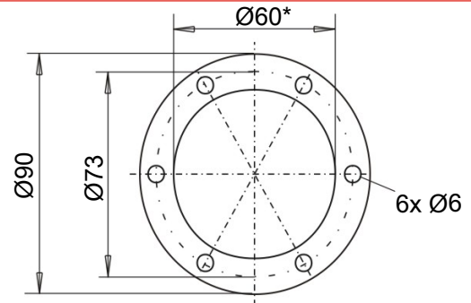
Flange drawing
