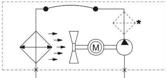
Standard version
