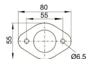
Adapter G3/4 to G1
