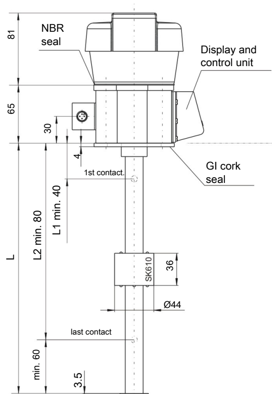
Flange drawing
