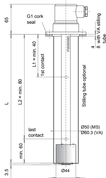
Basic model
