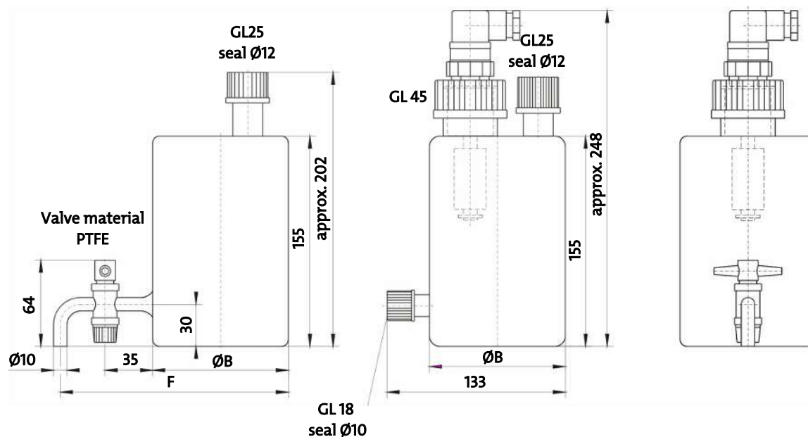
Model GL 3 with drain valve option
