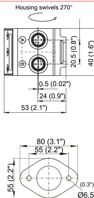
Flange drawing
