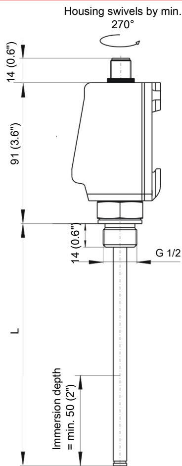
Side view
